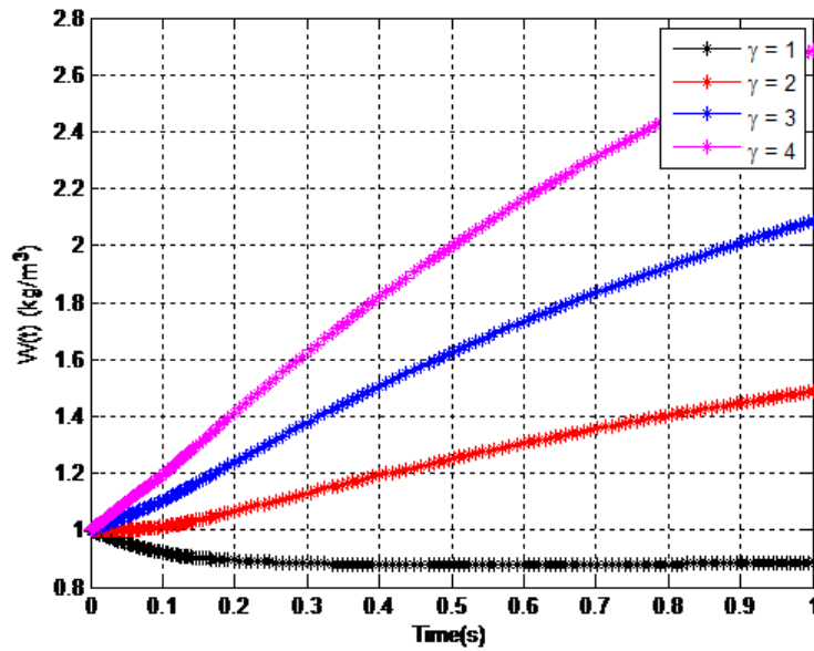
Figure 14. Variation in concentration of water droplet with time t for different values of the strength of formation of water droplets within the cloud, \gamma .
