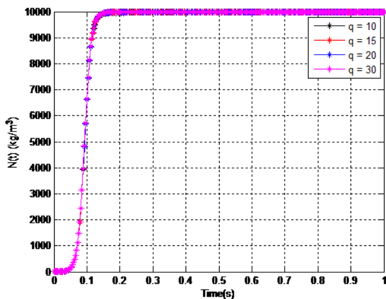
Figure 4. Variation of N with time t for different values of growth rate of rain, q .
