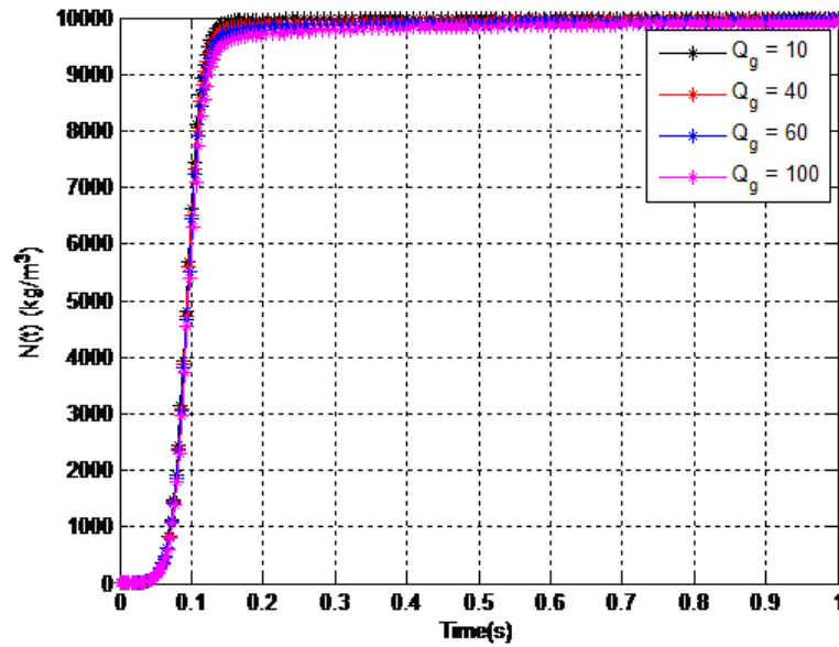
Figure 6. Variation of N with time t for different values of emission rates of gaseous pollutants, Q_g .
