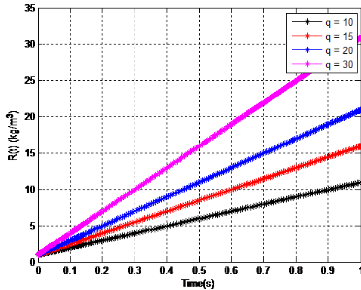
Figure 15. Variation of R with time t for different values of the growth rate of rain, q .
