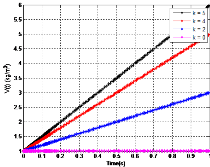
Figure 11. Variation of Water Droplet Number Density V(t) with Time for Zero formation of vapors, k .
