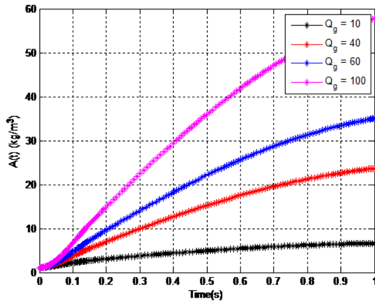
Figure 17. Variation in concentration of gaseous pollutant due to interaction with water vapor with time t for different values of gaseous emission rates, Q_g .
