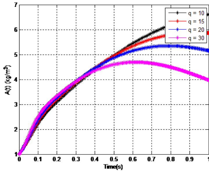
Figure 16. Concentration of gaseous pollutant due to interaction with water vapor against time t for different values of the growth rate of rain, q .
