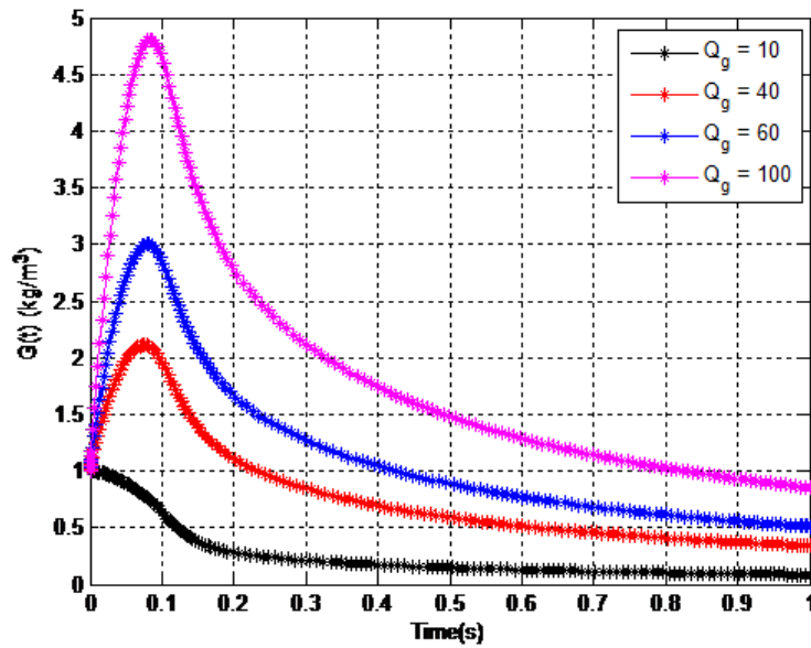
Figure 10. Variation of G with time t for different values of gaseous emission rates, Q_g .
