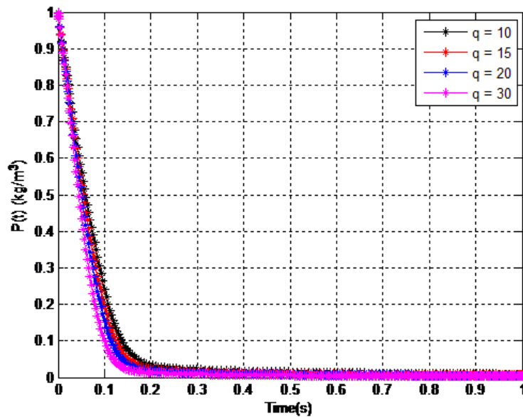
Figure 7. Variation of N with time t for different values value of growth rate of rain, q .
