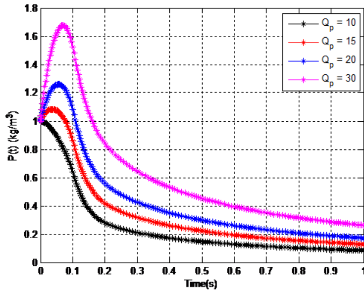
Figure 8. Variation of P with time t for different values of emission rates of particulate matters, Q_p .
