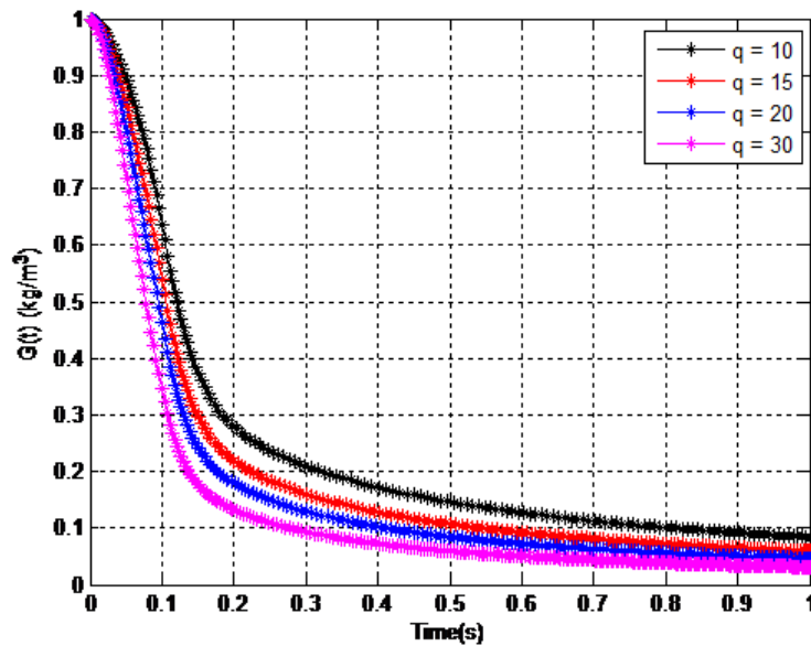
Figure 9. Graph of G with time t for different values of growth rate of rain, q .
