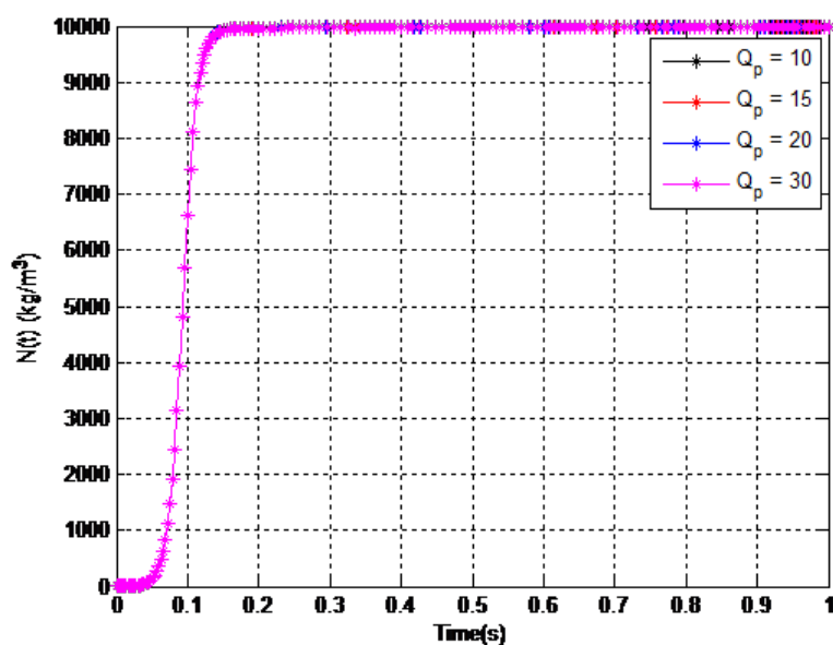
Figure 5. Variation of N with time t for different values of emission rates of particulate matters, Q_p .
