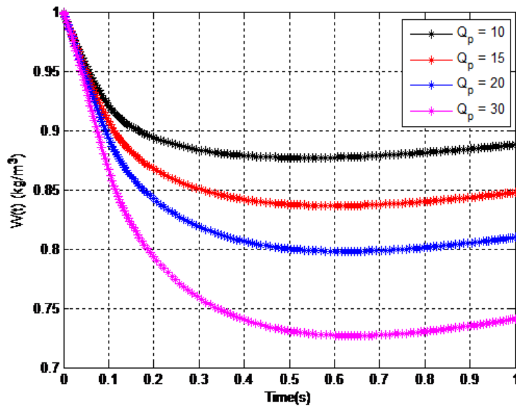
Figure 13. Variation of W with time t for different values particulate matters emission rates.
